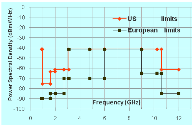
Figure 1: UWB emission masks in Europe [7] and the US [6]
