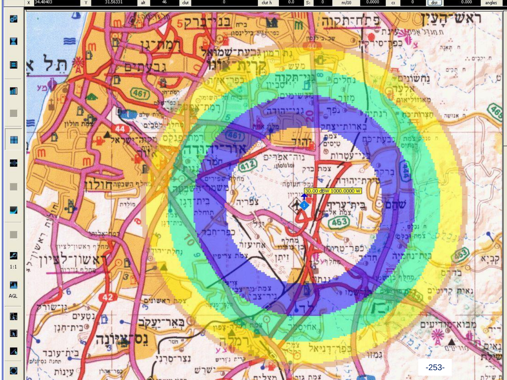
ATDI graph- Radar Coverage 5.5Ghz around BG airport
