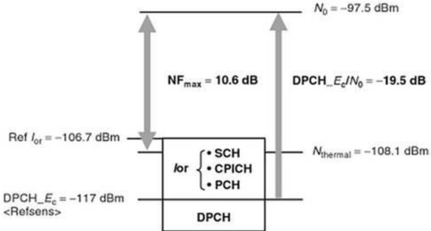
Figure 20.10 WCDMA band I reference sensitivity test case scenario (NF: Noise Figure; N_{\text{thermal}} : thermal noise power in 3.84 MHz bandwidth at 25 °C)
