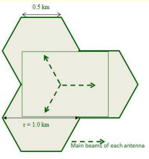
Tri-sector cells
