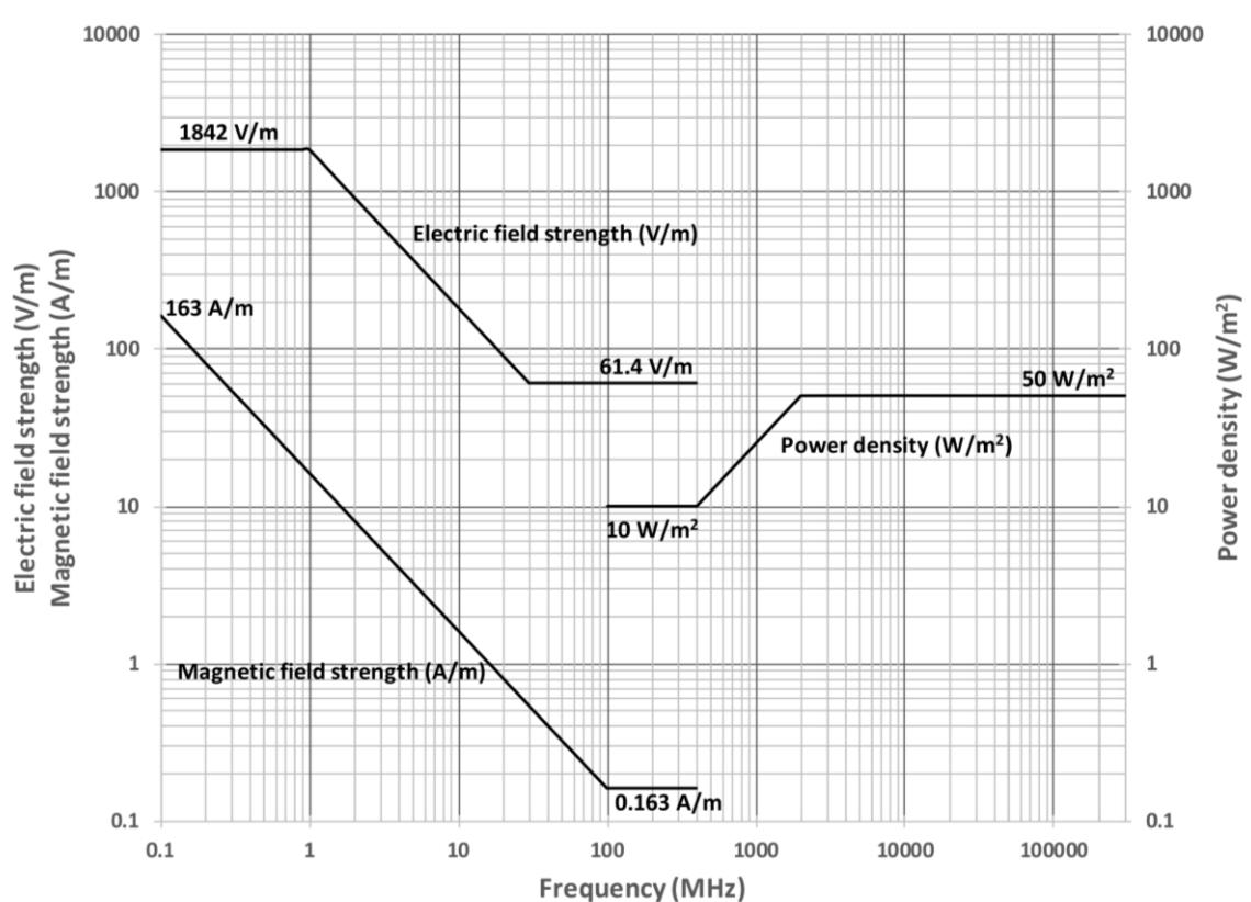
Figure 11 ( C95.1 2019 Fig. 4) EMFs and power density— restricted environments
